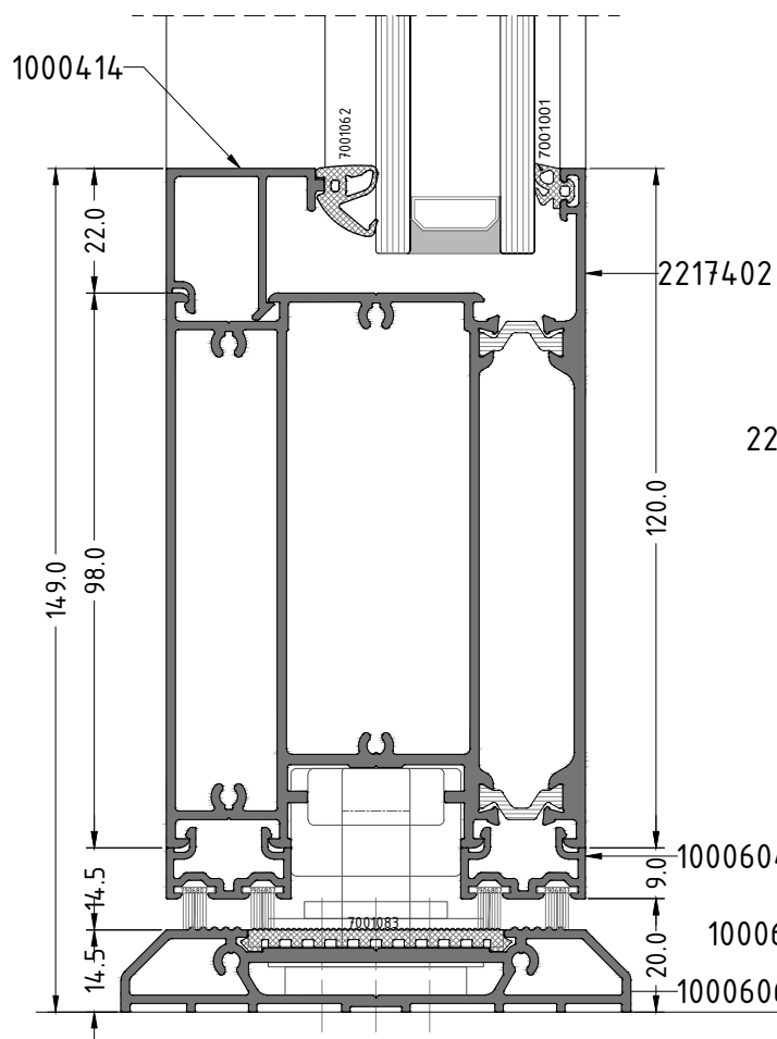
Section B With Threshold 1000606
