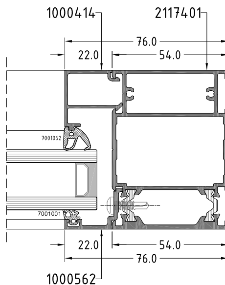
Section G
