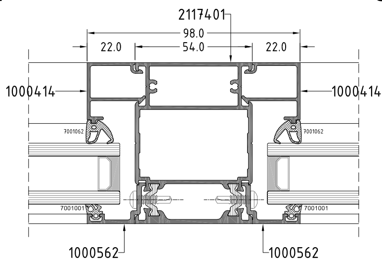
Section I
