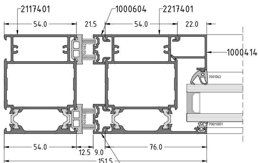
Section D
