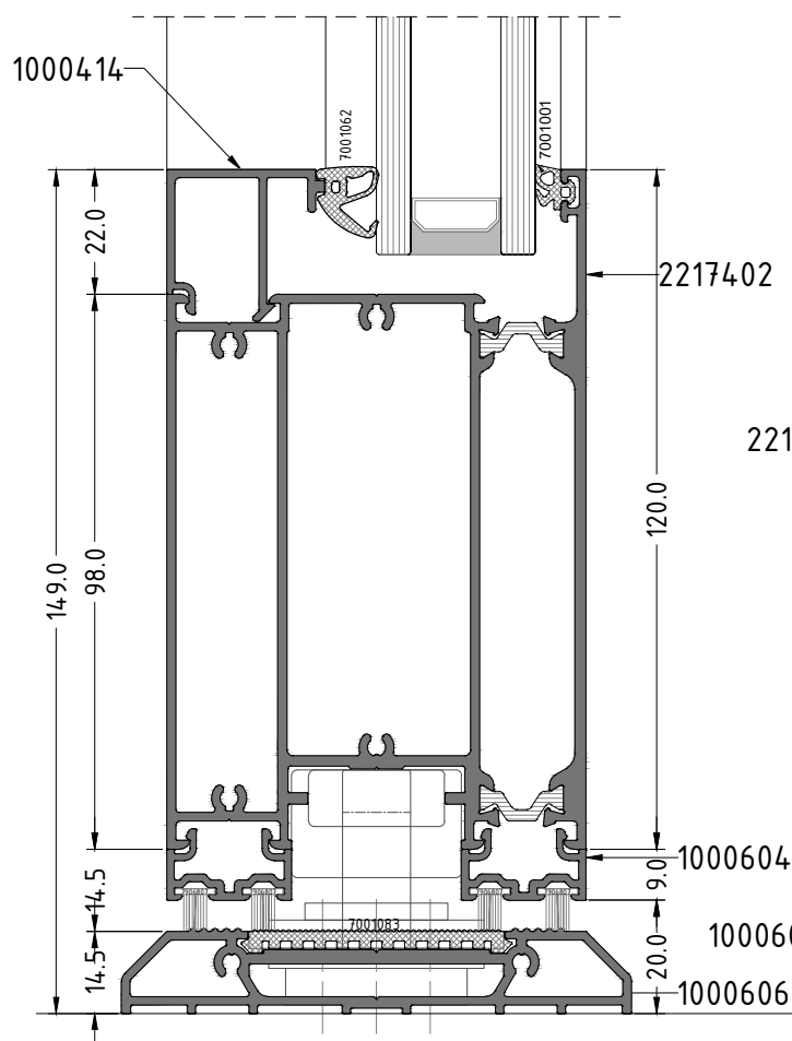
Section B
