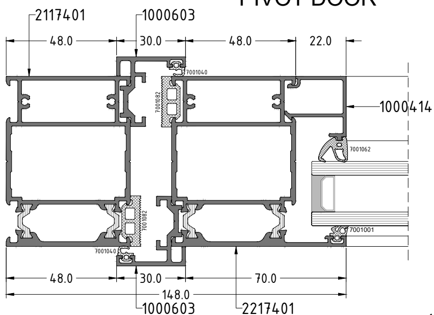
Section D
