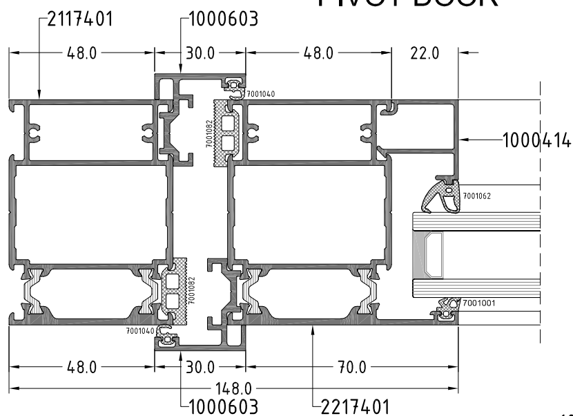
Section D
