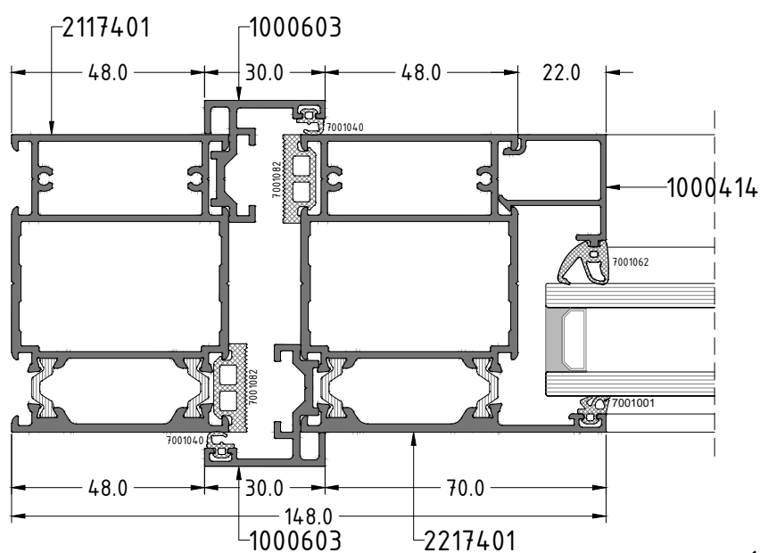
Section C
