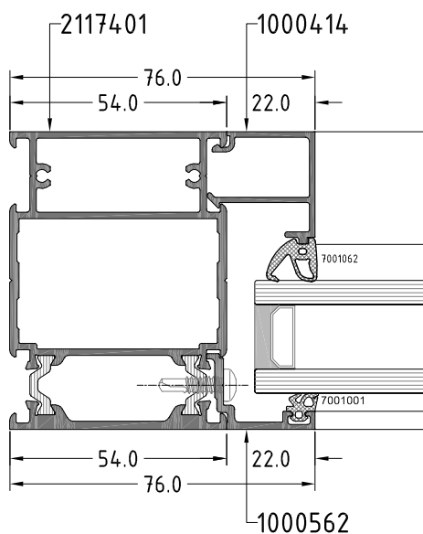
Section F
