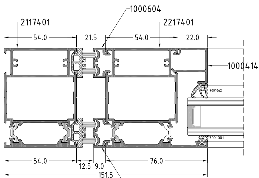
Section C
