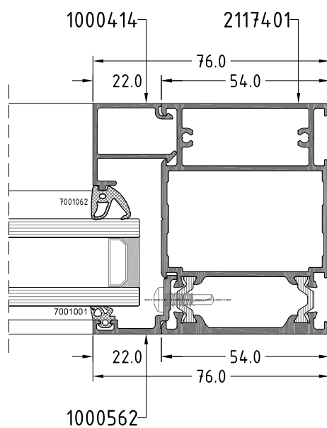
Section E
