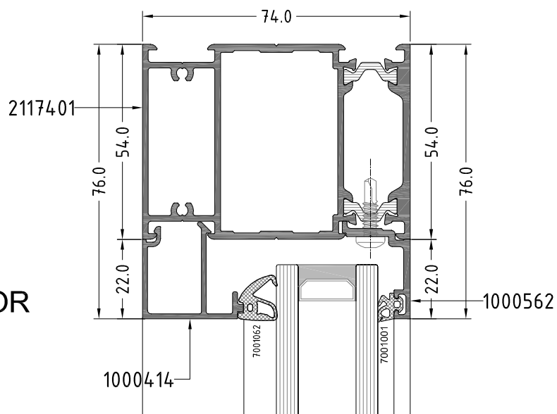
Section D
