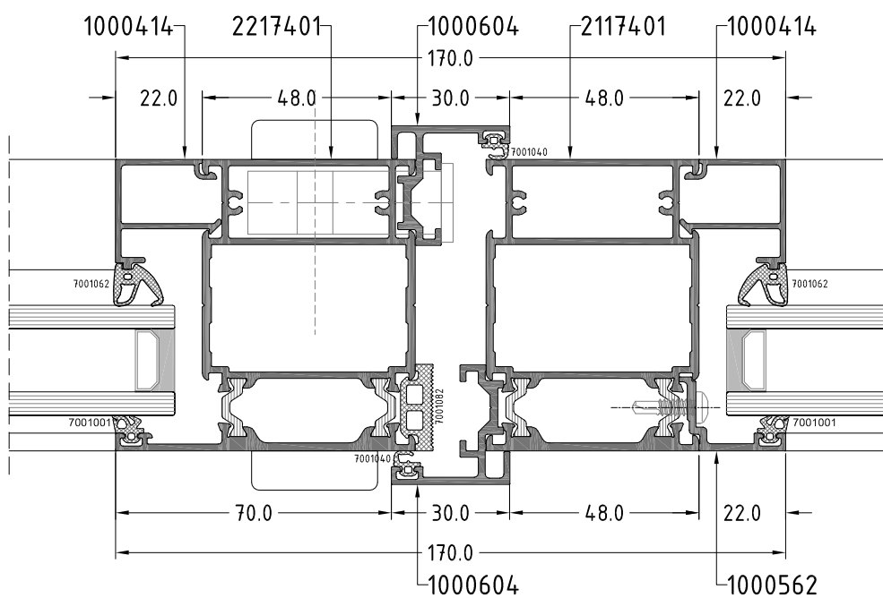
Section H
