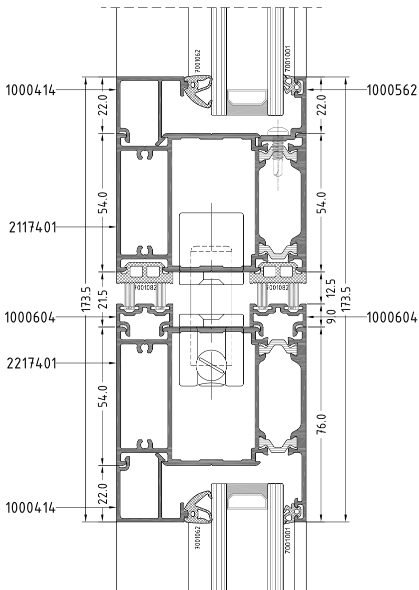
Section C
