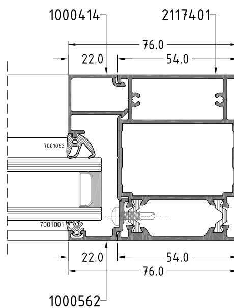
Section G
