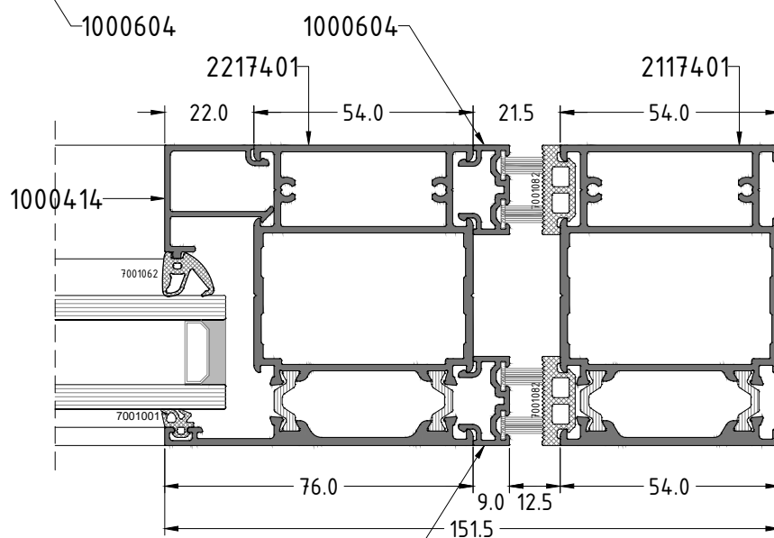
Section E
