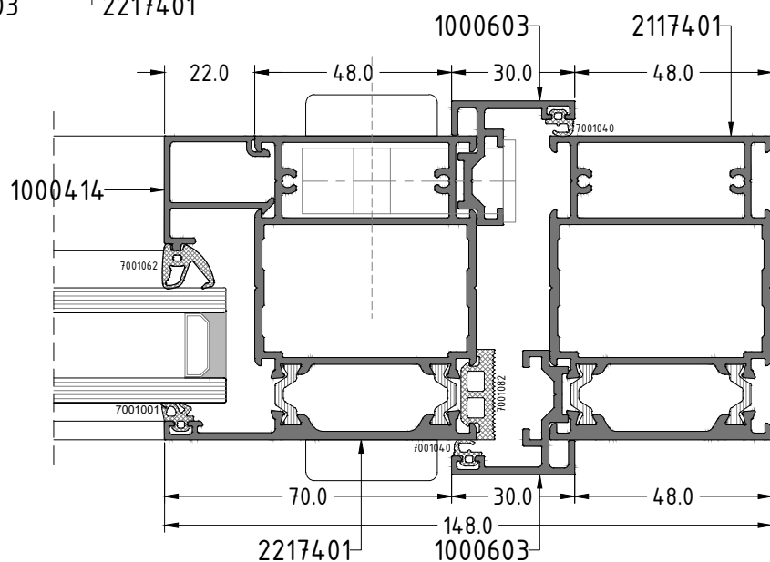
Section E
