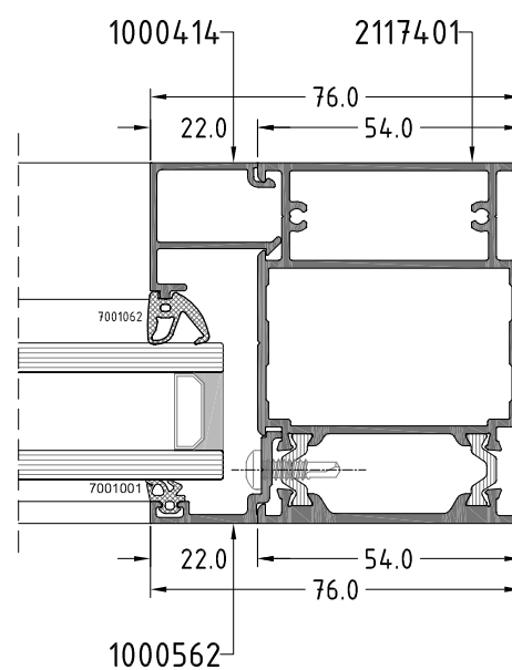
Section G
