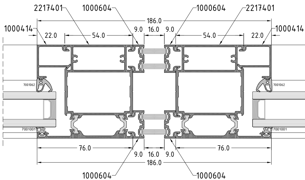
Section E
