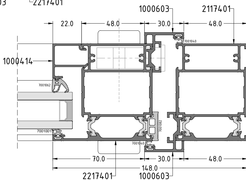
Section D
