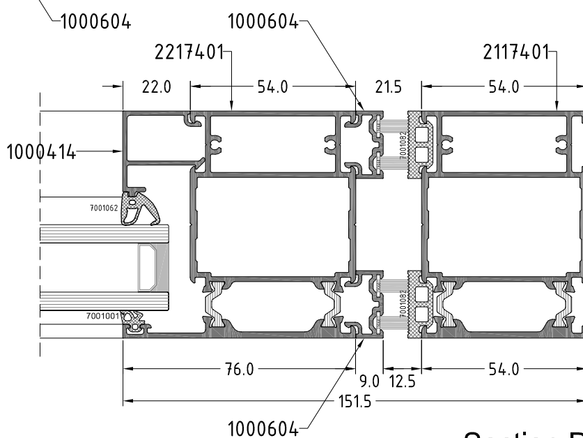
Section D
