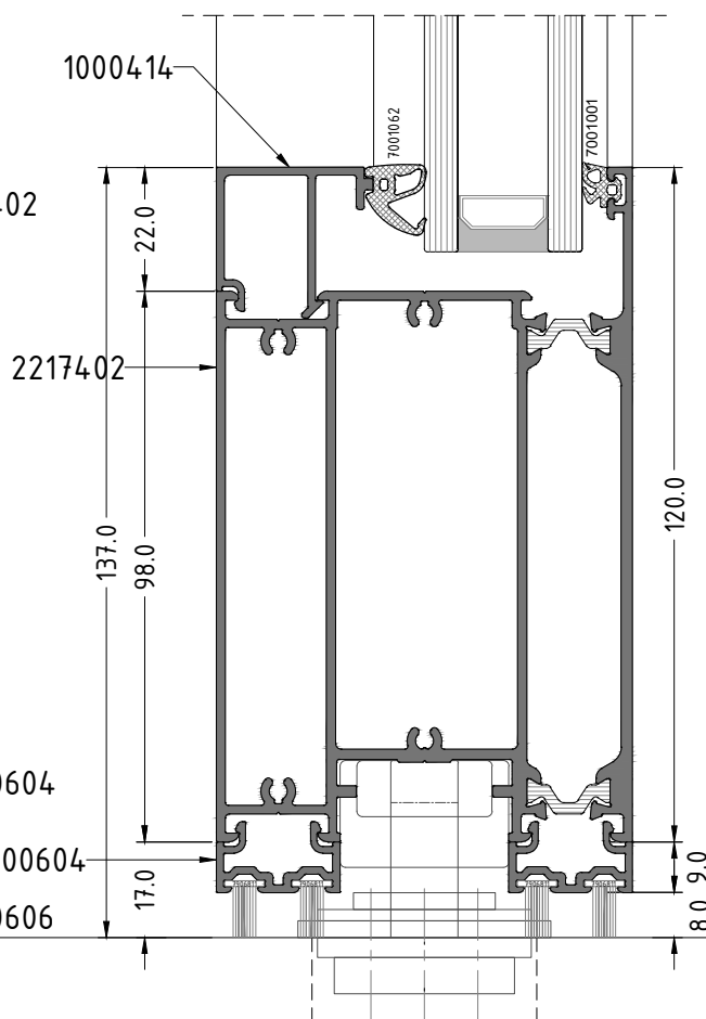
Section B
