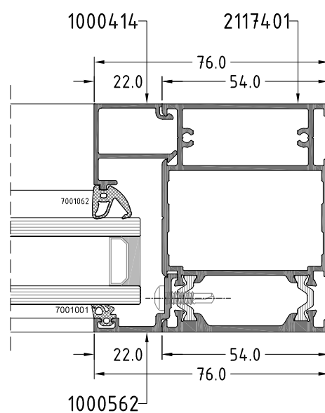
Section G
