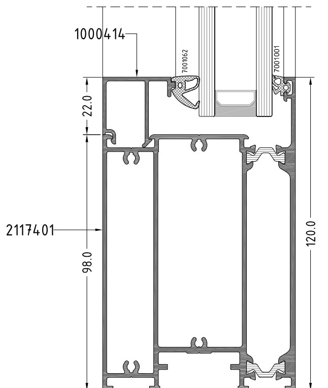
Section E
