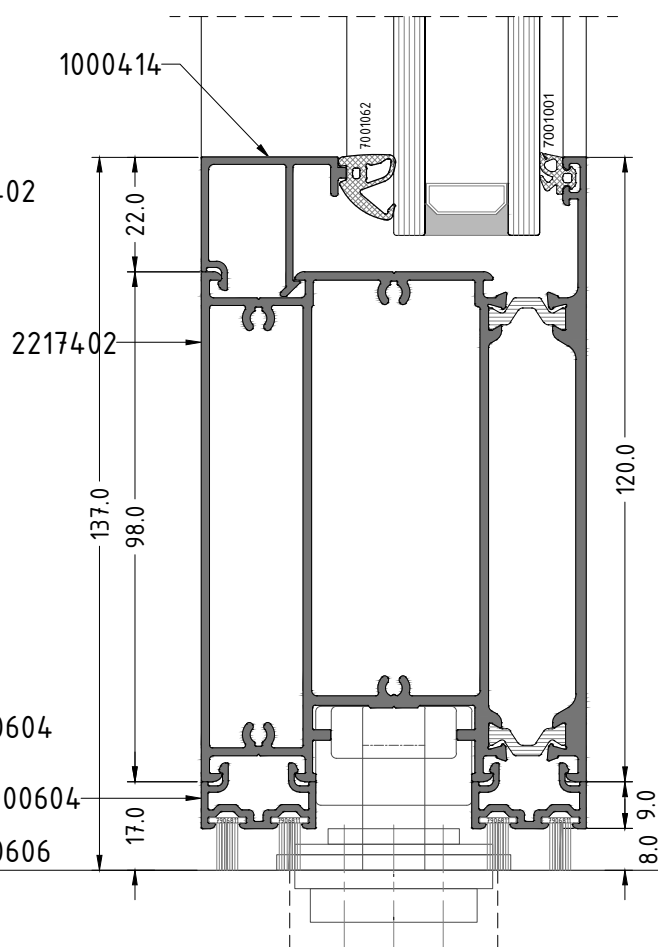
Section B Without Threshold
