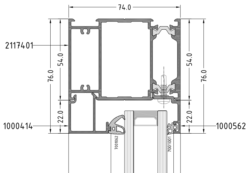
Section A
