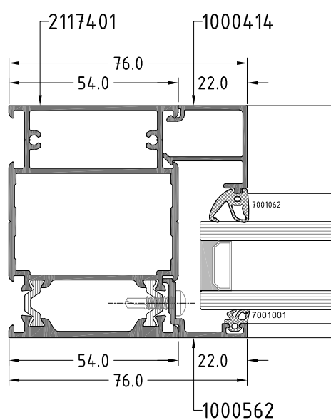
Section F
