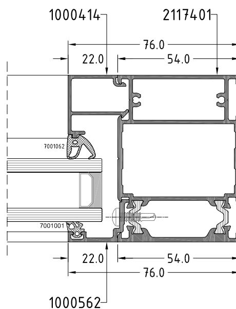
Section E
