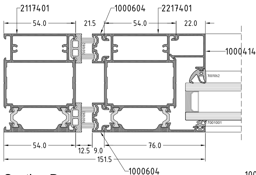
Section D
